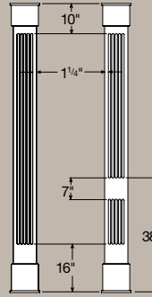
Flutes are 3/4" wide and 3/8" deep. Number and spacing of flutes varies by width of shaft.
