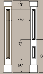
Route is 1 11/32" wide by 3/8" deep.
