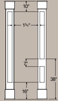
Recess is 5/8" deep and corners are 1/4" rounded.
